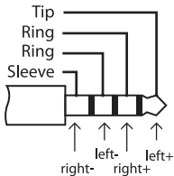
RE-600 Balanced Plug
